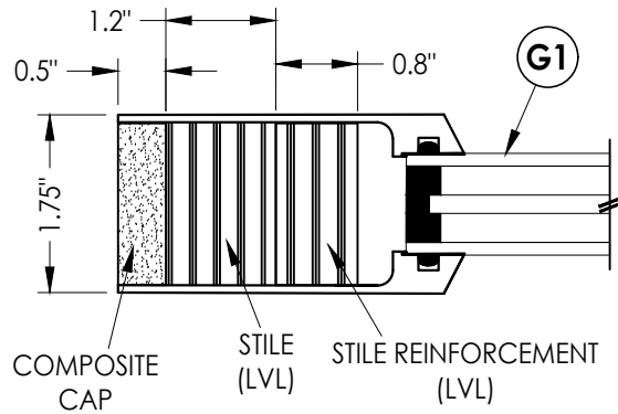
1 3 HORIZONTAL CROSS SECTION
