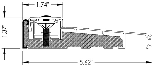
14 INSWING THRESHOLD Columbia
