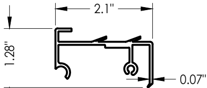
17 INSWING SIDELITE SPACER Columbia
